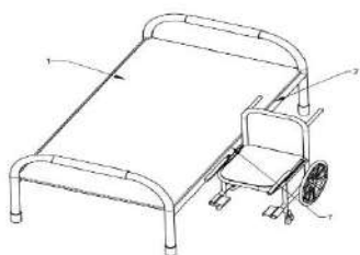
Title - Comfortable Cot with Wheel Chair Receptacle for Easy Transferring of Disabled Persons
