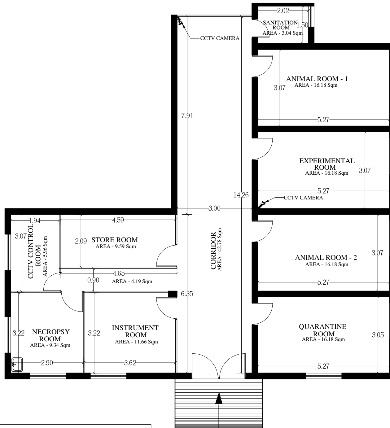
ANIMAL HOUSE - PROPOSED PLAN AREA - 151.28 Sqm (1627.8 Sft)
